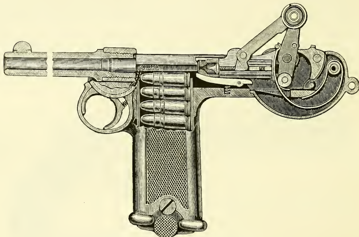
The Borchardt Automatic Magazine Pistol.
